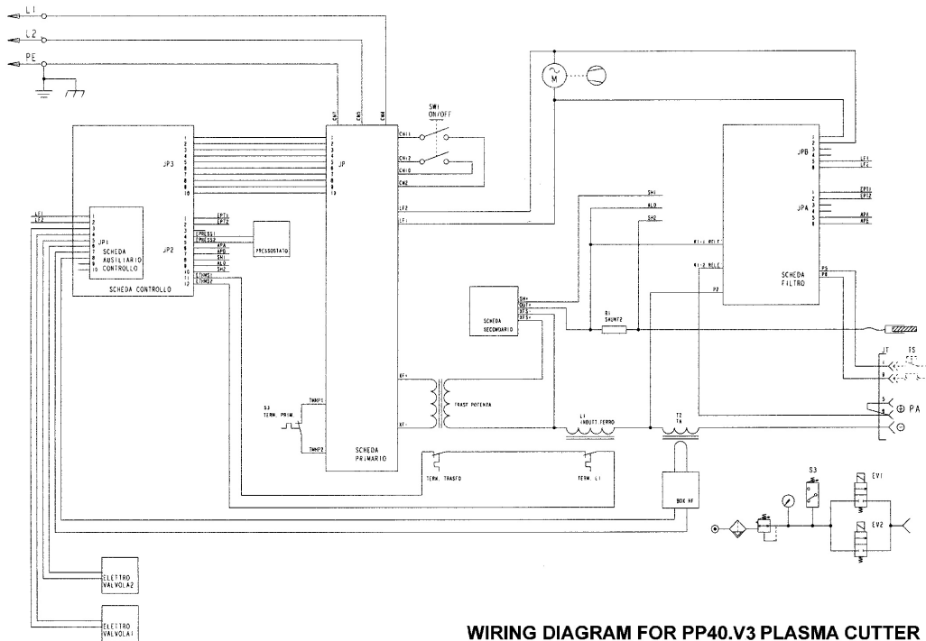
WIRING DIAGRAM FOR PP40.V3 PLASMA CUTTER
