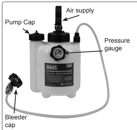
Brake and clutch bleeding system- Model No VS830
