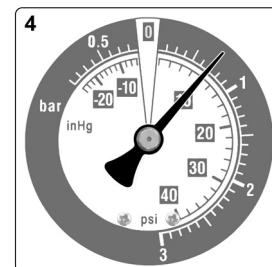
(4) READING: Reading low but steady DIAGNOSIS: Retarded ignition timing. Confirm using timing light and reset to manufacturer's specification.
