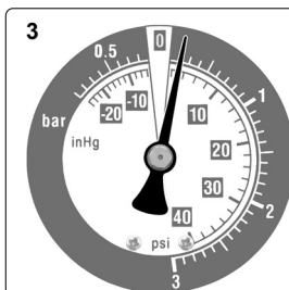
(3) READING: Extremely low but steady DIAGNOSIS: Leaking intake manifold system, Faulty manifold gasket or carburettor base gasket, split vacuum hose, seized open EGR valve.
