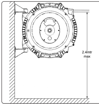
Wall Mounting
