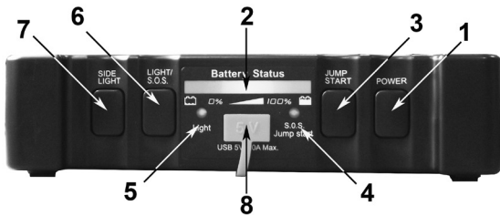
fig.1 Front Panel
