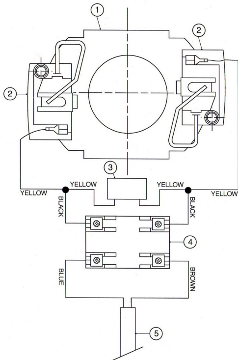
WIRING DIAGRAM T20K
