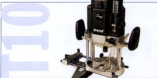
An adjustable inner plate ensures that subsequent guidebush fittings are accurate
