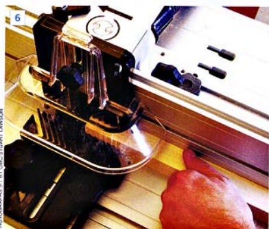
Profiling using the pressure fingers
