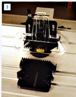
The guard plus the vertical and horizontal pressure fingers in place
