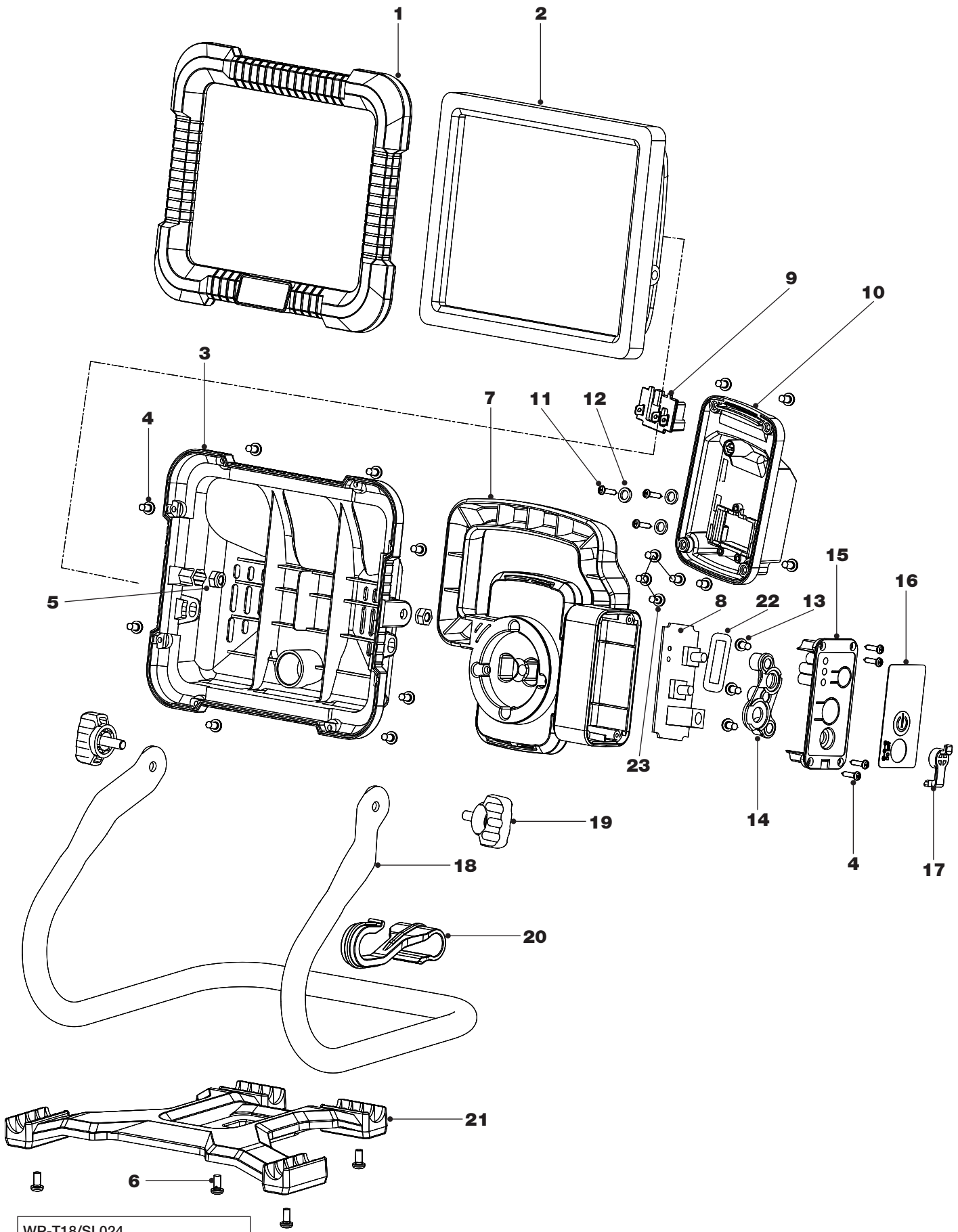
WP-T18/SL024 Base Plate Assembly - 6 (x4), 21
