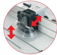
Guard assembly Quick lateral and height adjustment of finger pressure and guard.
