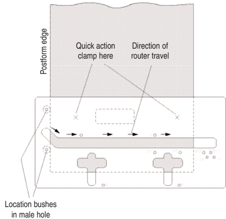
Location bushes in male hole
