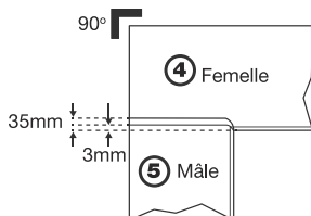
Raccord (3mm-35mm Encastrement)
