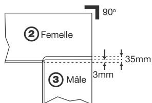
Raccord (3mm-35mm Encastrement)
