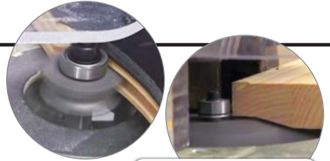
The scribe is cut on the end grain of the timber.
